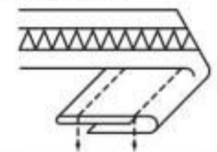
KHF83 繡縫車細條面貼器 Tape Attach Folder for Covering Stitch
