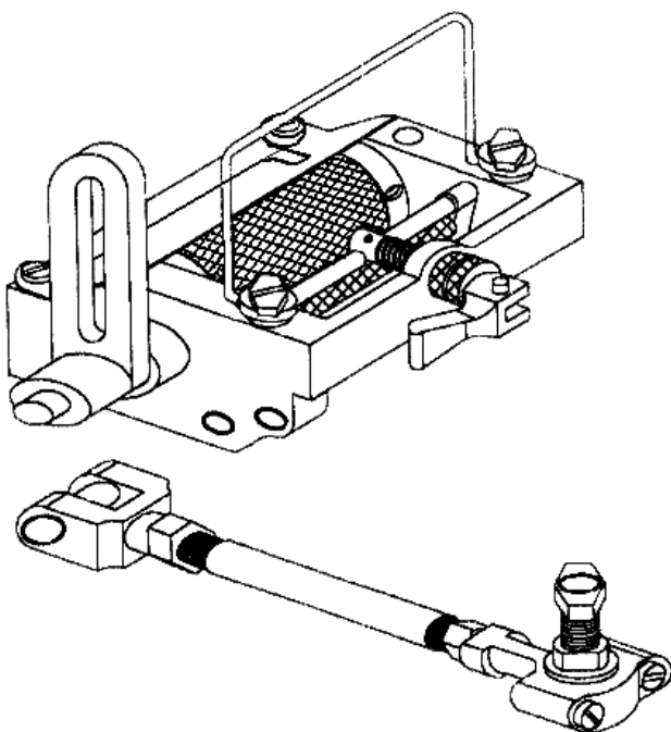
Front Elastic Feeder with Connecting Assembly 前送料器及連結組件
